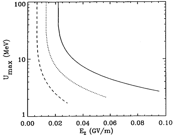
FIG. 12. Plot of maximum electron energy versus accelerating gradient for the parameters in Fig. 9 with a = 3 mm (solid curve), 5 mm (dotted curve), and 10 mm (dashed curve).
