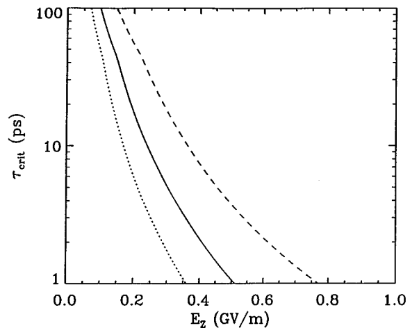
FIG. 7. Plot of critical pulse time \tau_{\text{crit}} versus the accelerating gradient E_z for a laser of wavelength \lambda = 10 \mu\text{m} . The dielectric constant \epsilon = 1.5 (dotted curve), 3 (solid curve), 9 (dashed curve). The other parameters are the same as in Fig. 6 with U_I = 8 \text{ eV} .
