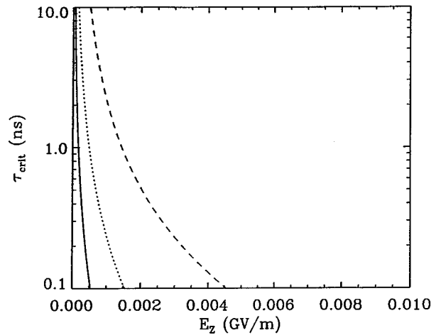
FIG. 15. Plot of critical pulse time \tau_{\text{crit}} versus the accelerating gradient E_z in a gas- (helium-) filled ICA with laser wavelength \lambda = 1 mm. The gas pressures and corresponding wall radii are 3 atm and 26.5 mm (solid curve), 10 atm and 14.5 mm (dotted curve), and 30 atm and 8.4 mm (dashed curve), with U_I = 24.6 eV, \nu_m/P_g = 10^{12} sec ^{-1} /atm, and \nu_0/P_g = (2m/M)\nu_m/P_g = 3 \times 10^8 sec ^{-1} /atm.
