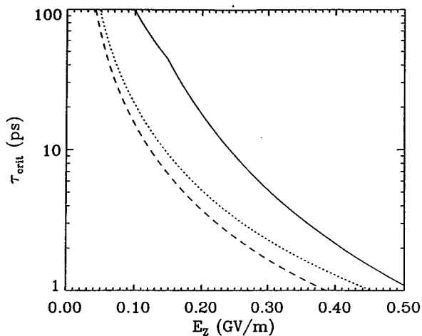
FIG. 5. Plot of critical pulse time \tau_{\text{crit}} versus the accelerating gradient E_z for a laser of wavelength \lambda = 10 \mu\text{m} . The initial electron density n_{p0} is 0 (solid curve), 1 \text{ cm}^{-3} (dotted curve), and 10^5 \text{ cm}^{-3} (dashed curve). In addition, a = 30 \mu\text{m} , b = 80 \mu\text{m} , \epsilon = 3 , U_I = 8 \text{ eV} , \nu_m = 10^{15} \text{ sec}^{-1} , and \nu_0 = 10^{11} \text{ sec}^{-1} .
