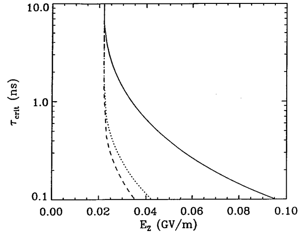
FIG. 10. Plot of critical pulse time \tau_{\text{crit}} versus the accelerating gradient E_z for a millimeter wave driver, \lambda=1 \text{ mm} . The initial electron density n_{p0} is 0 (solid curve), 1 \text{ cm}^{-3} (dotted curve), and 10^5 \text{ cm}^{-3} (dashed curve). The parameters are the same as in Fig. 9, with a=3 \text{ mm} and b=8 \text{ mm} .
