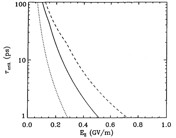
FIG. 6. Plot of critical pulse time \tau_{\text{crit}} versus the accelerating gradient E_z for a laser of wavelength \lambda = 10 \mu\text{m} . The ionization potential U_I = 4 \text{ eV} (dotted curve), 8 \text{ eV} (solid curve), 12 \text{ eV} (dashed curve). The other parameters are the same as in Fig. 5 with n_{p0} = 0 .
