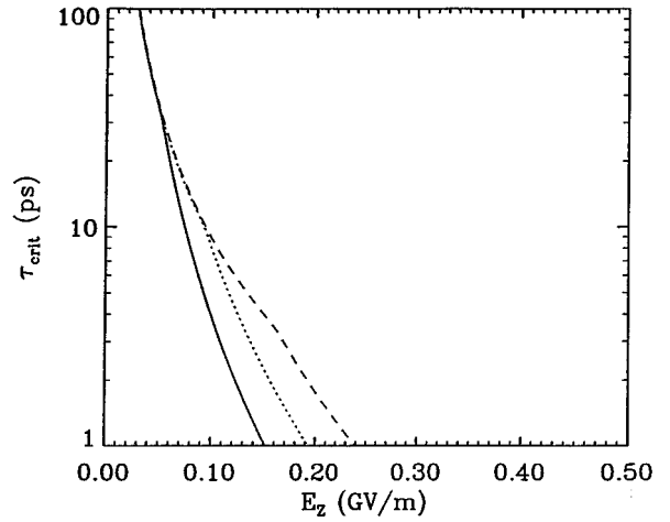
FIG. 14. Plot of critical pulse time \tau_{\text{crit}} versus the accelerating gradient E_z in a gas- (helium-) filled ICA with laser wavelength \lambda = 10 \mu\text{m} . The gas pressures and corresponding wall radii are 3 atm and 265 \mu\text{m} (solid curve), 10 atm and 145 \mu\text{m} (dotted curve), and 30 atm and 84 \mu\text{m} (dashed curve), with U_I = 24.6 eV, \nu_m/P_g = 10^{12} sec ^{-1} /atm, and \nu_0/P_g = (2m/M)\nu_m/P_g = 3 \times 10^8 sec ^{-1} /atm.
