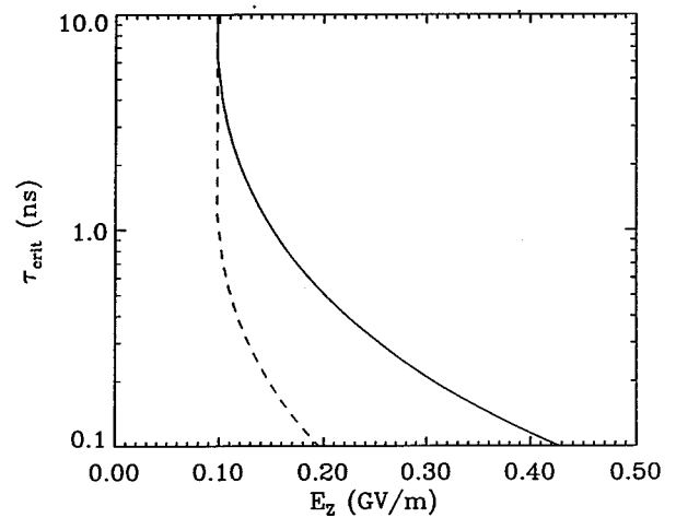
FIG. 11. Plot of critical pulse time \tau_{\text{crit}} versus the accelerating gradient E_z for a millimeter wave driver, \lambda=1 \text{ mm} . The initial electron density n_{p0} is 0 (solid curve) and 1 \text{ cm}^{-3} (dashed curve). The parameters are a=0.2 \text{ mm} , b=0.283 \text{ mm} , \epsilon=10 , U_I=8 \text{ eV} , \nu_m=10^{15} \text{ sec}^{-1} , and \nu_0=10^{11} \text{ sec}^{-1} .
