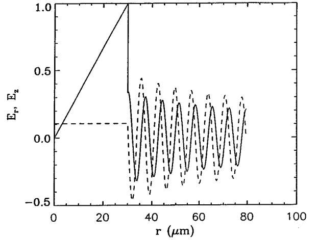
FIG. 2. Axial and radial components of the electric field for a dielectrically lined waveguide supporting an axially symmetric TM mode with phase velocity equal to c . The solid (dotted) curve denotes the radial (axial) component of the electric field normalized to the peak radial field at r = a . The parameters are \lambda = 10 \mu\text{m} , a = 30 \mu\text{m} , b - a = 50 \mu\text{m} , and \epsilon = 3 .
