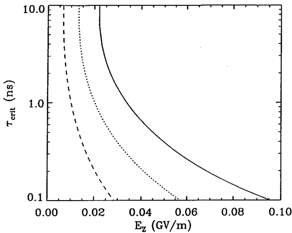
FIG. 9. Plot of critical pulse time \tau_{\text{crit}} versus the accelerating gradient E_z for a millimeter wave driver, \lambda=1 \text{ mm} . The inner radius a=3 \text{ mm} (solid curve), 5 \text{ mm} (dotted curve), and 10 \text{ mm} (dashed curve), where b-a=5 \text{ mm} . In addition, \epsilon=3 , U_I=8 \text{ eV} , n_{p0}=0 , \nu_m=10^{15} \text{ sec}^{-1} , and \nu_0=10^{11} \text{ sec}^{-1} .
