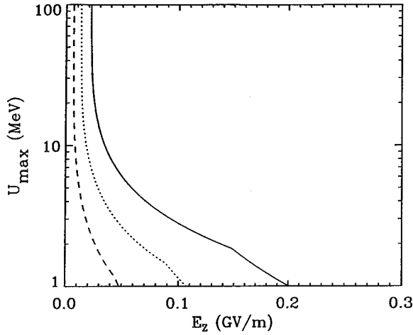
FIG. 8. Plot of maximum electron energy versus accelerating gradient for the parameters in Fig. 4 with a=30 \mu\text{m} (solid curve), 50 \mu\text{m} (dotted curve), and 100 \mu\text{m} (dashed curve).
