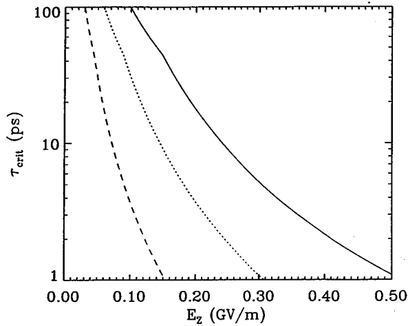
FIG. 4. Plot of critical pulse time \tau_{\text{crit}} versus the accelerating gradient E_z for a laser of wavelength \lambda = 10 \mu\text{m} , inner radius a = 30 \mu\text{m} (solid curve), 50 \mu\text{m} (dotted curve), and 100 \mu\text{m} (dashed curve), b - a = 50 \mu\text{m} . In addition, \epsilon = 3 , U_I = 8 \text{ eV} , n_{p0} = 0 , \nu_m = 10^{15} \text{ sec}^{-1} , and \nu_0 = 10^{11} \text{ sec}^{-1} .
