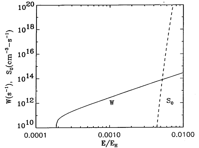
FIG. 3. Plot of tunneling ionization source function S and collisional ionization rate W as a function of normalized electric field \tilde{E} = E / E_H . In this plot U_I = 8 \text{ eV} , \lambda = 10 \mu\text{m} , \nu_m = 10^{15} \text{ sec}^{-1} , and \nu_0 = 10^{11} \text{ sec}^{-1} .
